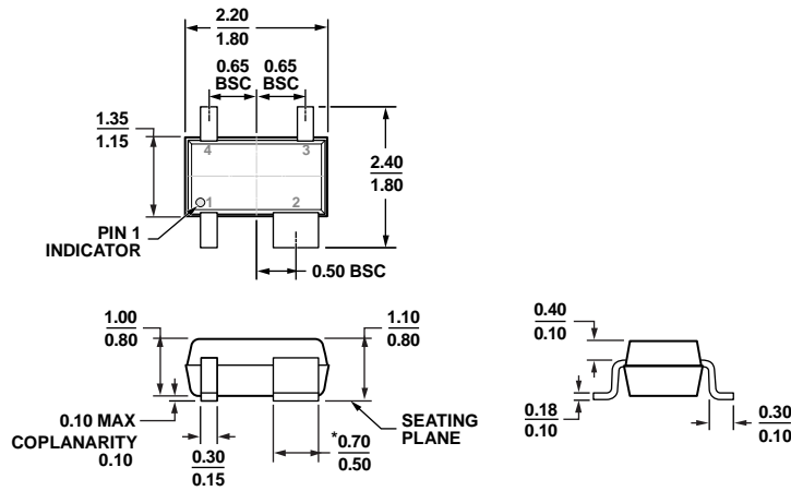
*PACKAGE OUTLINE CORRESPONDS IN FULL TO EIAJ SC82 EXCEPT FOR WIDTH OF PIN 2 AS SHOWN. Figure 22. 4-Lead Thin Shrink Small Outline Transistor Package [SC70] (KS-4) Dimensions shown in millimeters
